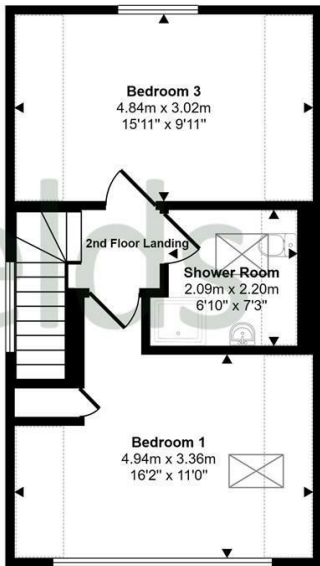
Second Floor Approx 43 sq m / 466 sq ft
